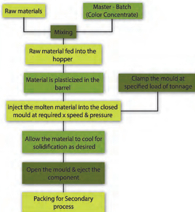
Flow Process Diagram 1.1 Injecting Molding Process:
